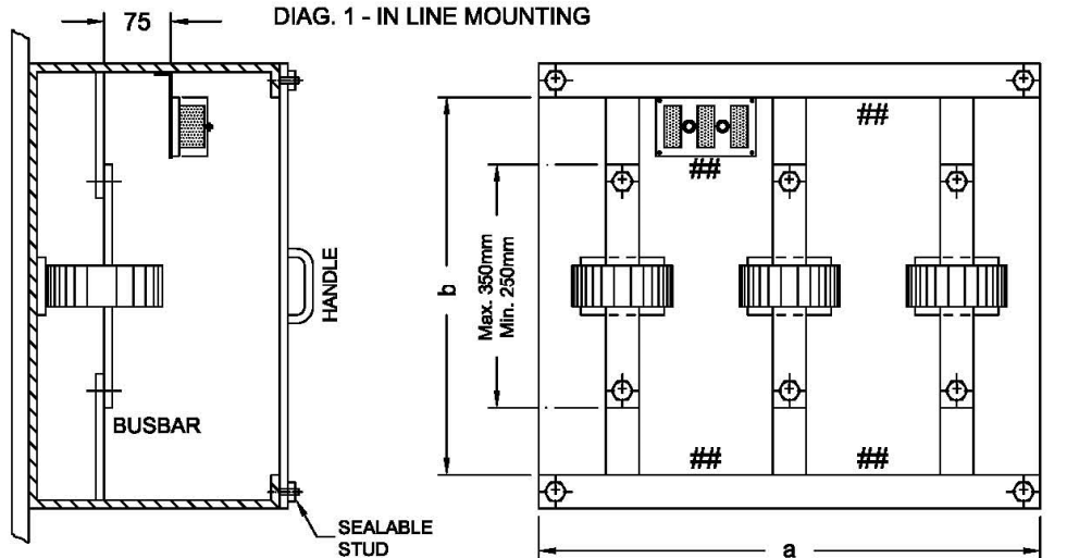
DIAG. 1 - IN LINE MOUNTING
