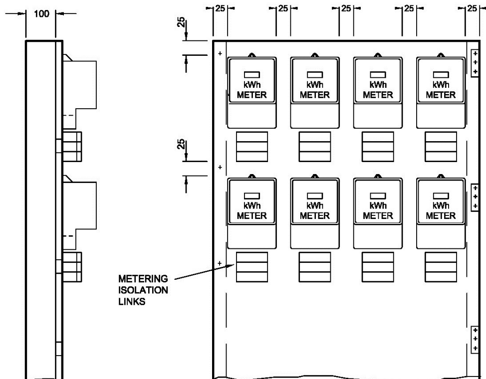
VIEWS SHOWING HINGED PANEL MOUNTING ARRANGEMENTS
