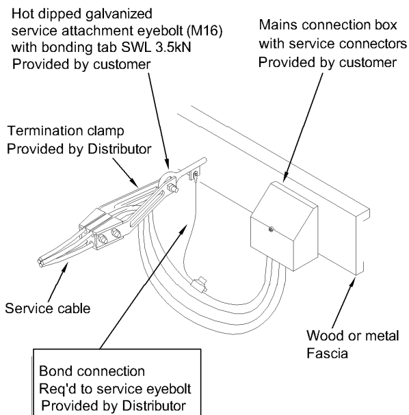
50/95 sqmm LV ABC SERVICE CONNECTION WOOD OR METAL FASCIA - 3.5kN SWL
