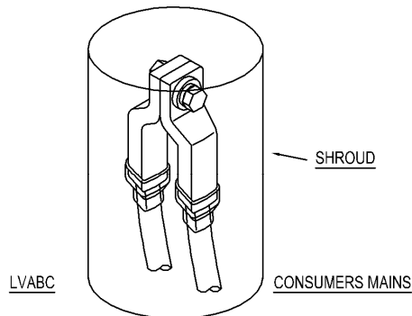
LVABC PHASE CONNECTION TO SINGLE CUSTOMER'S MAINS
