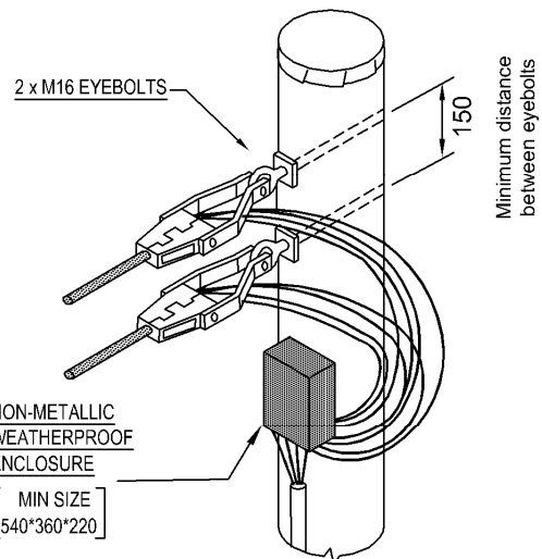
TWIN 50/95 sqmm LVABC SERVICE CONNECTION CUSTOMER'S WOOD POLE
