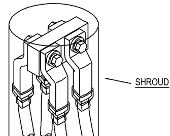
TWIN 50/95 sqmm LVABC SERVICE CONNECTION CUSTOMER'S WOOD POLE
