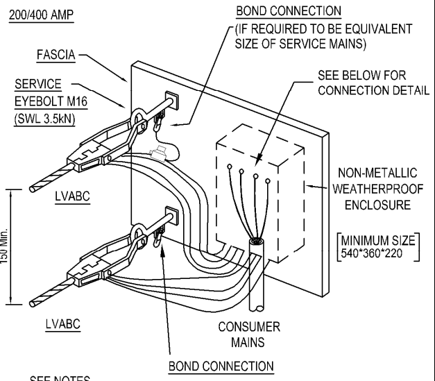
TYPICAL TWIN LVABC SERVICE TO CUSTOMER'S MAINS CONNECTION DETAIL
