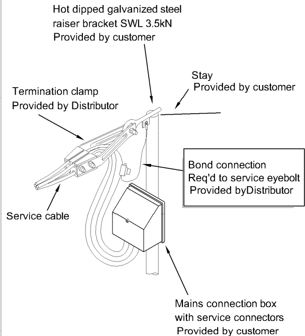
50/95 sqmm LV ABC SERVICE CONNECTION GALVANISED STEEL RISER BRACKET - 3.5kN SWL
