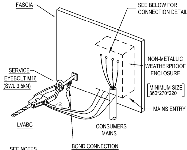
TYPICAL SINGLE LVABC SERVICE TO CUSTOMER'S MAINS CONNECTION DETAIL
