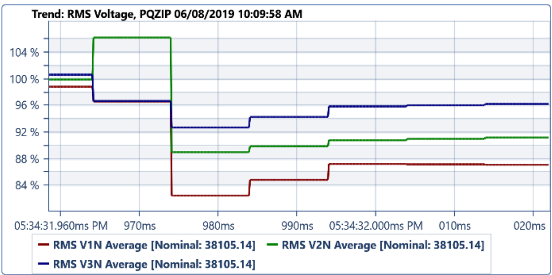
Figure 18: Measured 66kV rms voltages
