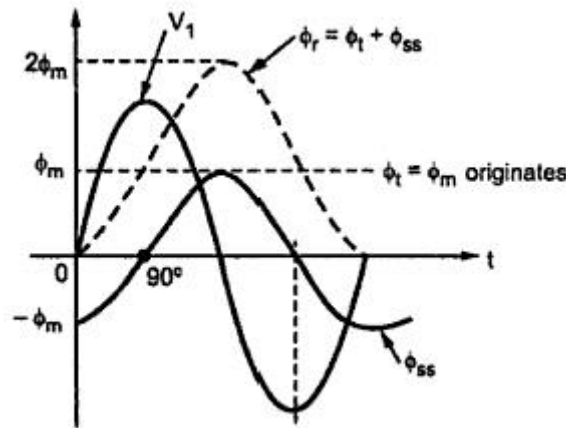
Figure 9: Doubling Effect in a Transformer (Your Electrical Home 2013)
