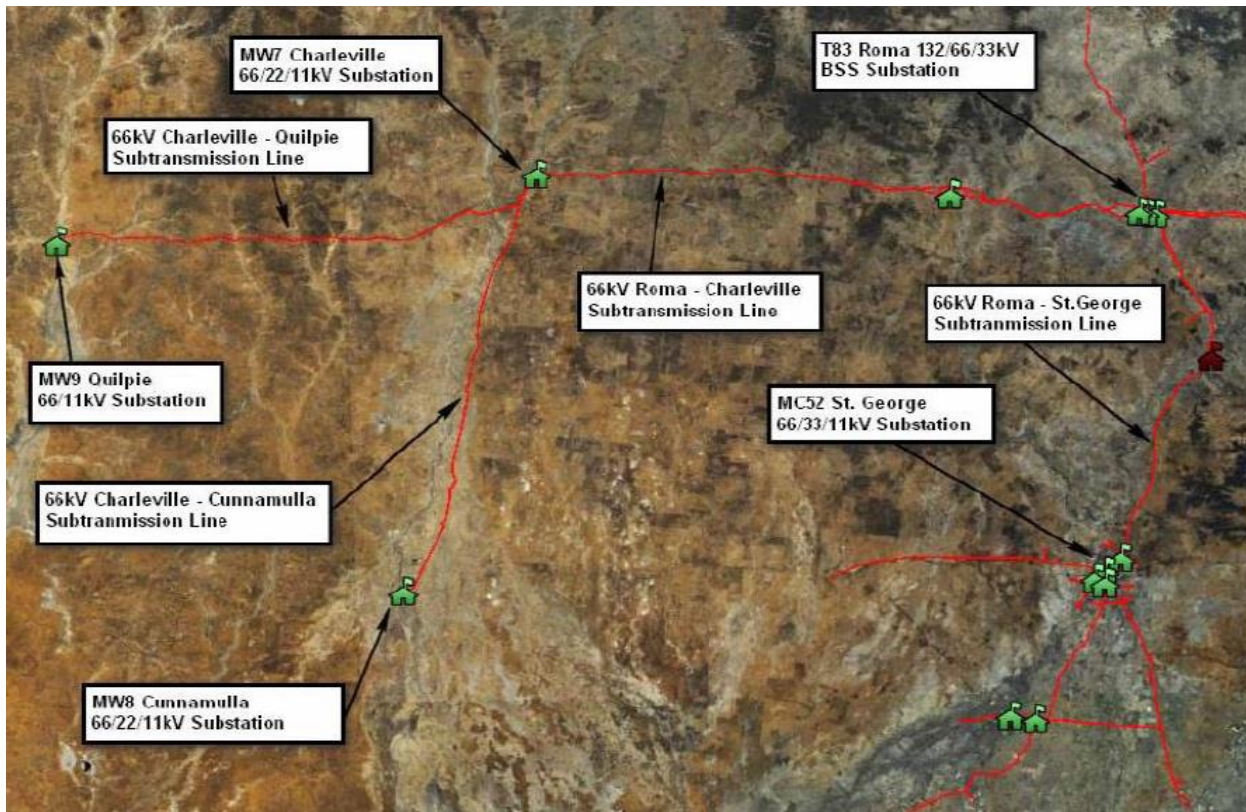
Figure 1 – Charleville Subtransmission System
