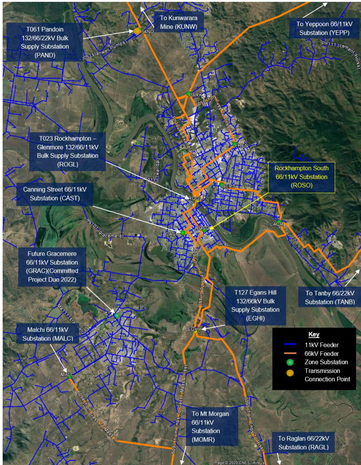
Figure 1: Existing network arrangement (geographic view)
