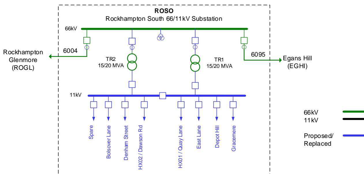
Figure 10: Option 1 proposed network arrangement (schematic view)
