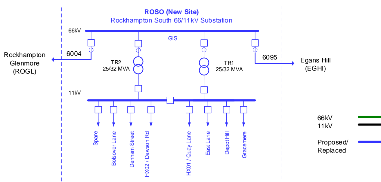
Figure 11: Option 2 proposed network arrangement (schematic view)
