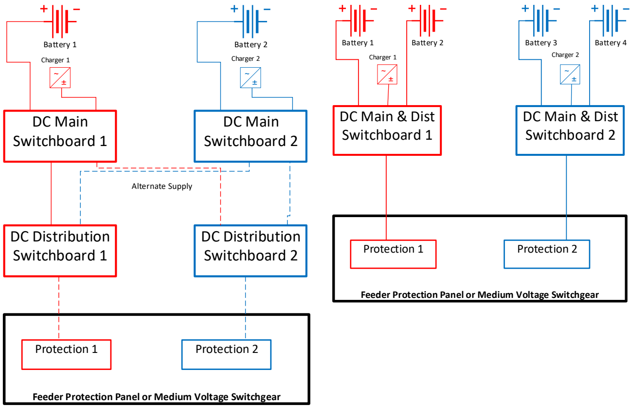
Existing Energex Dual DC Supply Scheme
