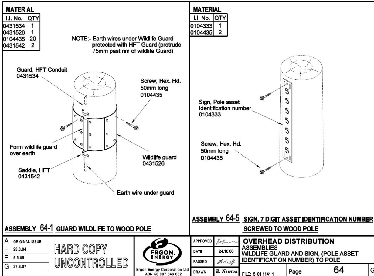
Figure 7. Assembly 64
